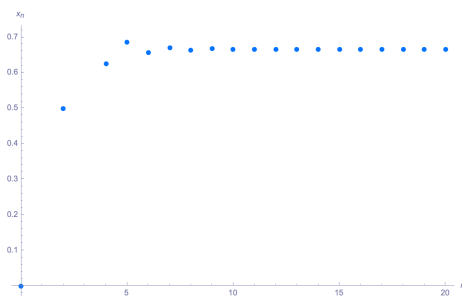
Fig. 3.2: x_{n+2} = x_{n+1} + x_n
