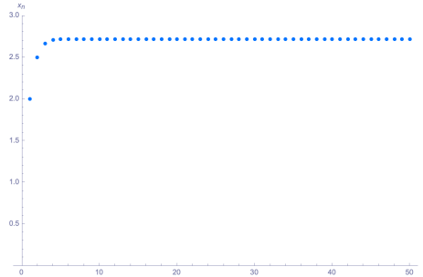
Fig. 3.1: y_n = (1 + \frac{1}{n})^n
