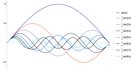
Fig. 8.3: f_n(x) = \frac{\sin nx}{n} for 1 \leq n \leq 8 .
